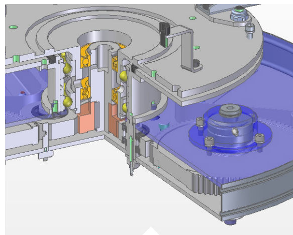
FULL METAL GEAR BOX. PLANETARY HEAD that is 100% tempered metal and geared driven not belt.
